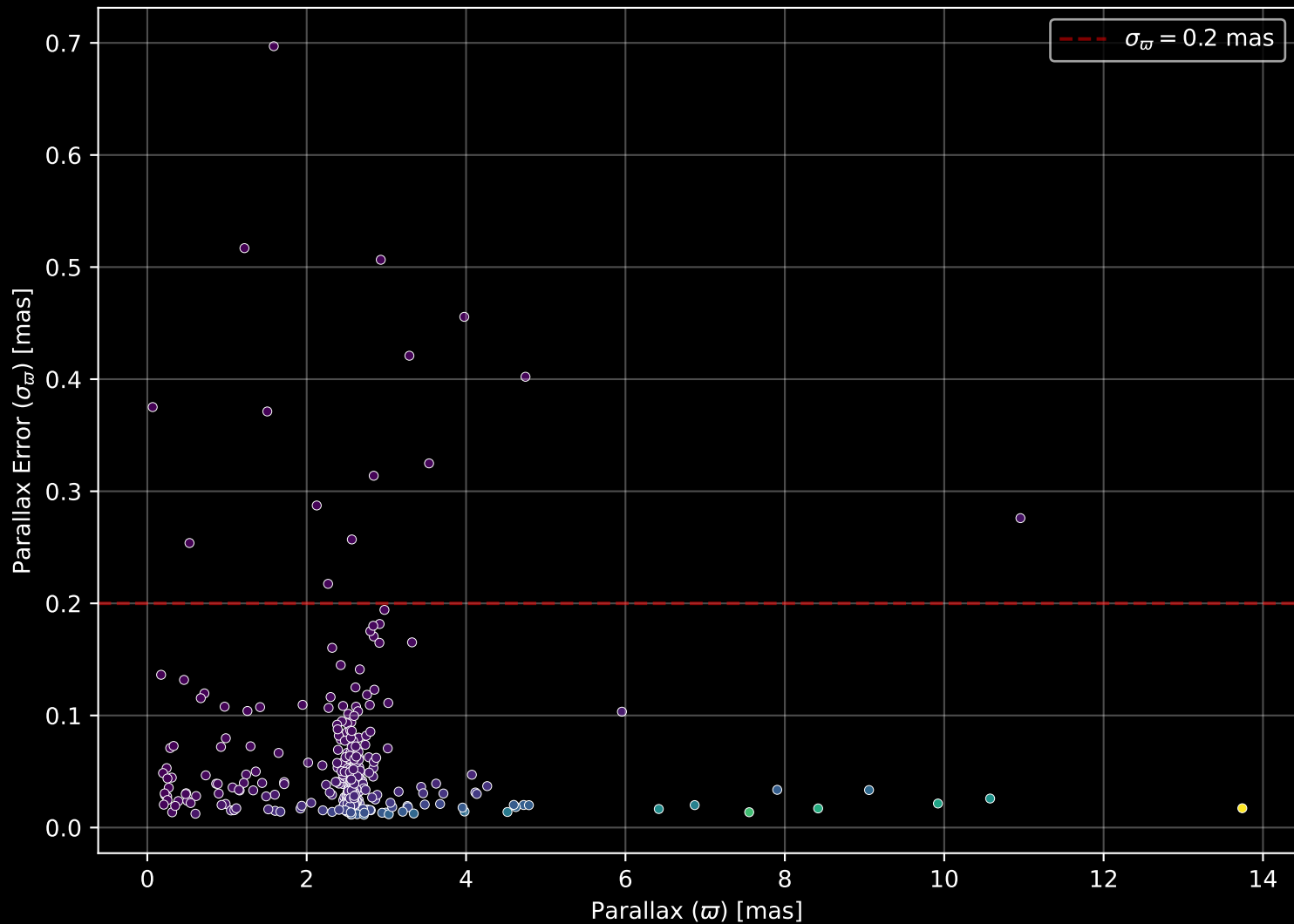
APOGEE DR17 Field: [ORIONA] Parallax Quality (n= 396)
