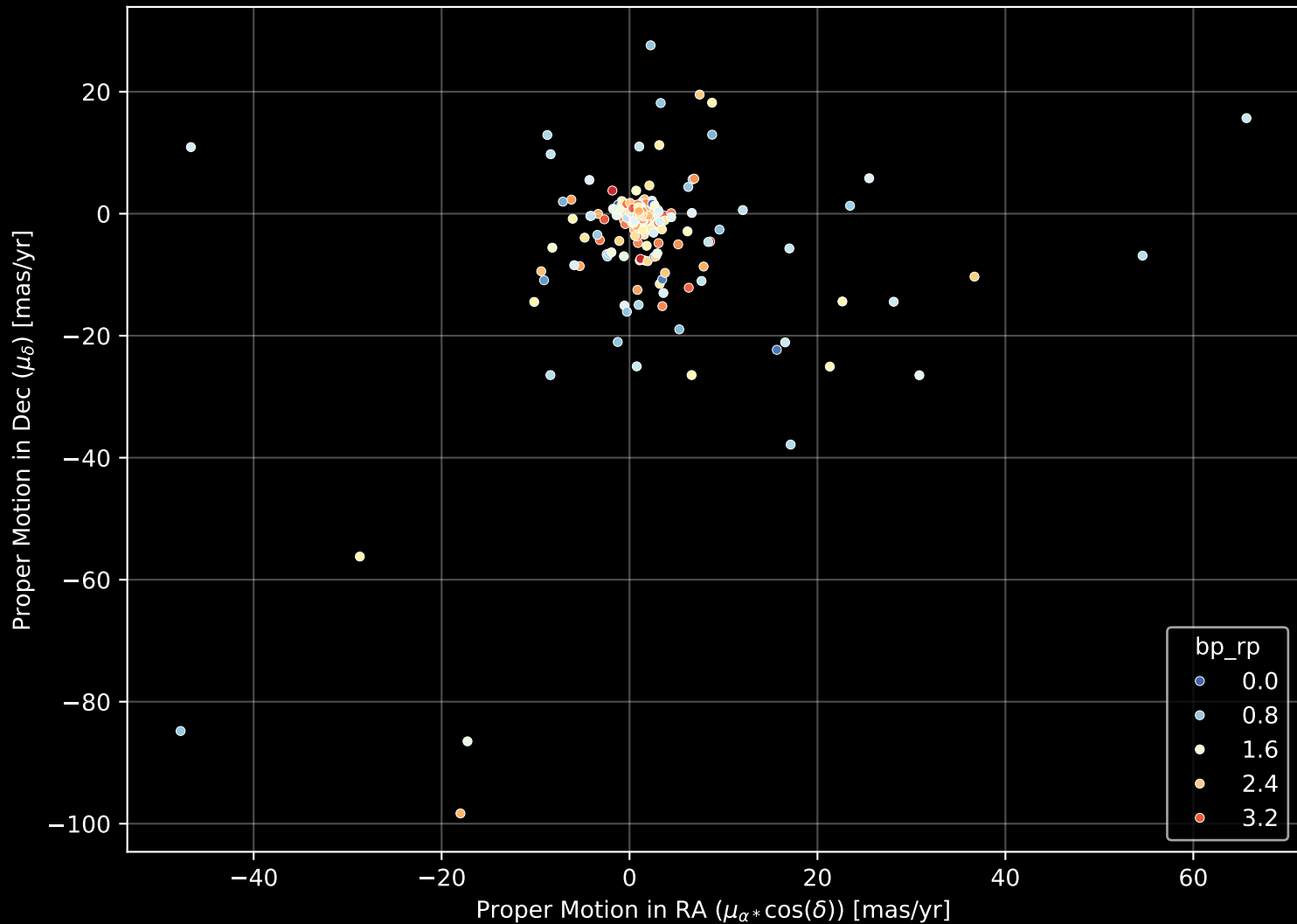
APOGEE DR17 Field: [ORIONA] Proper Motion Diagram (n= 396)
