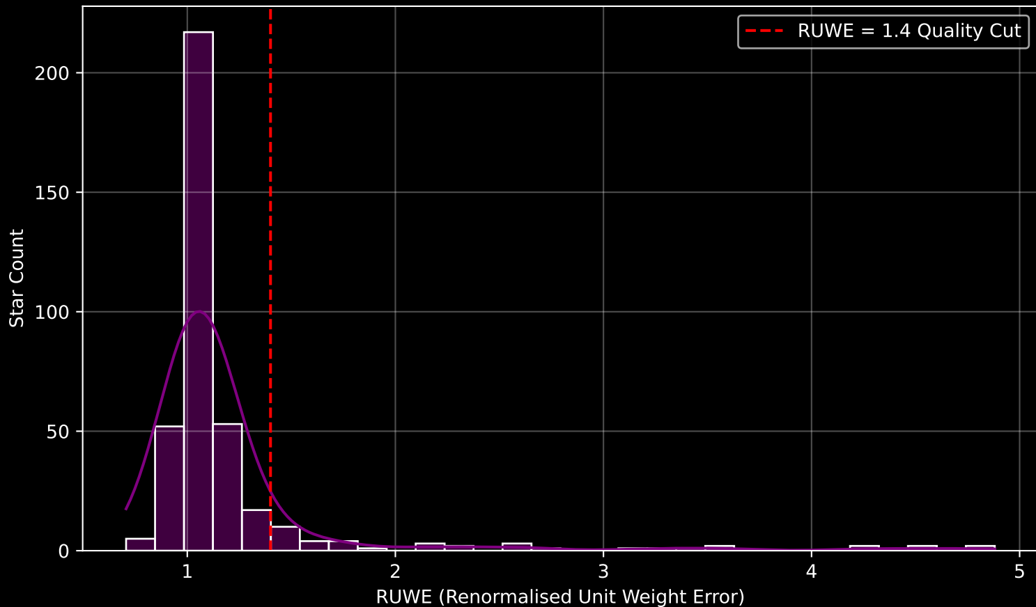
GAPOGEE DR17 Field [ORIONA] RUWE Distribution (n= 383)
