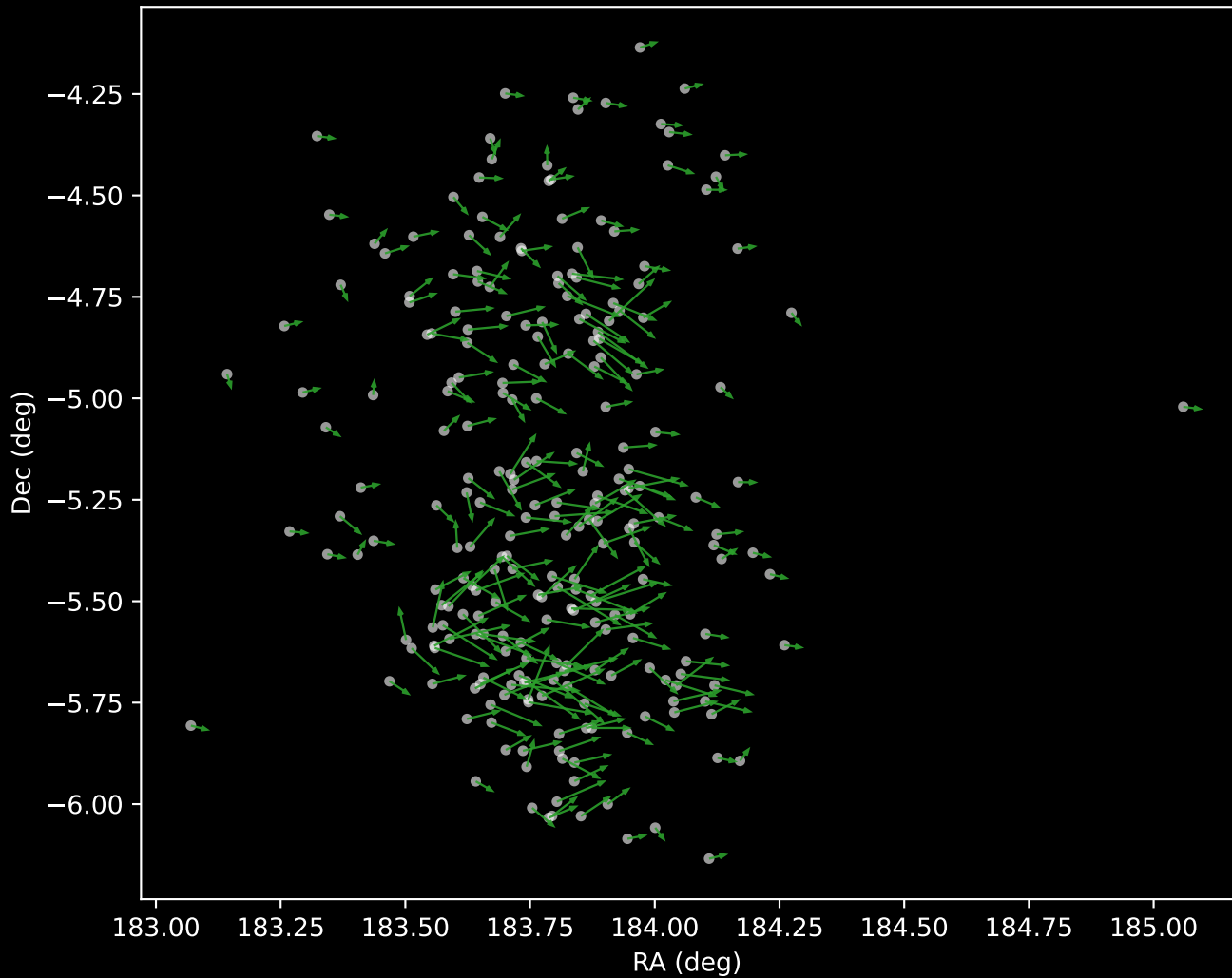
APOGEE DR17 Cluster 4 Proper Motion Vectors (n=244)
