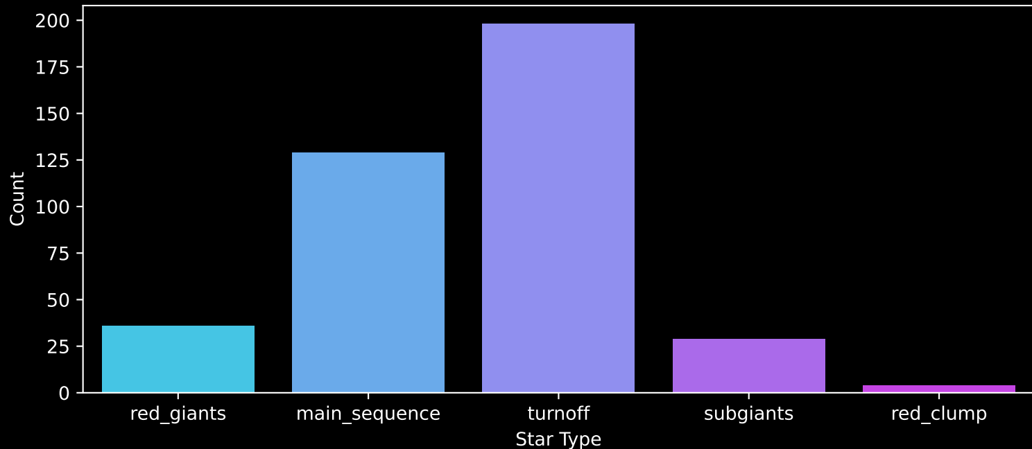
APOGEE DR17 Field: [ORIONA] Count plot of Star Type
