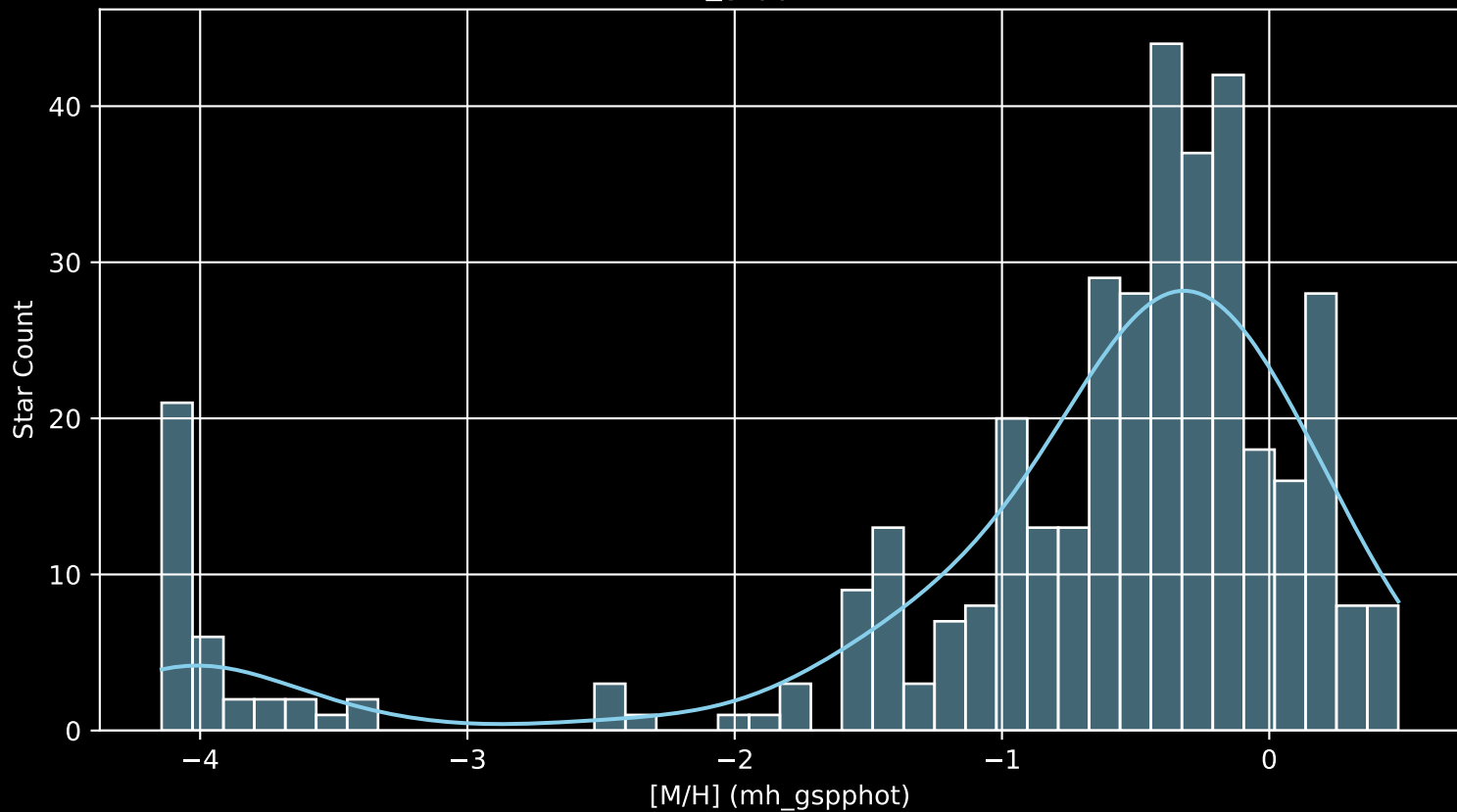
APOGEE DR17 Field: [ORIONA [M/H] (mh_gspphot) (n= 389)
